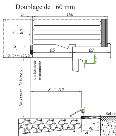
Doublage de 100 mm, 120 mm, 140 mm, 160 mm
